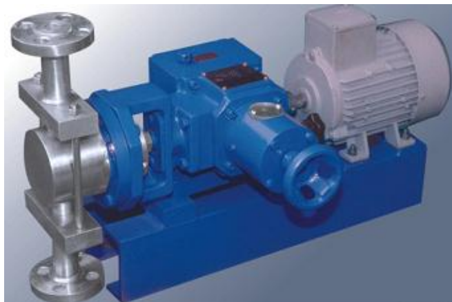
Receprocating pump
