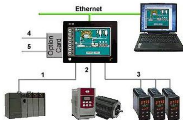
Simple system with protocol conversion
